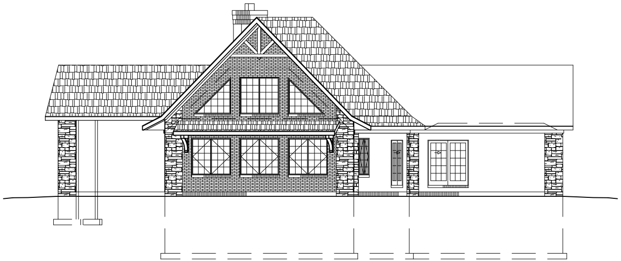
1 SOUTH ELEVATION A-1
